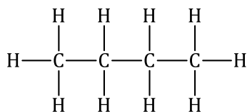
n-Butane
